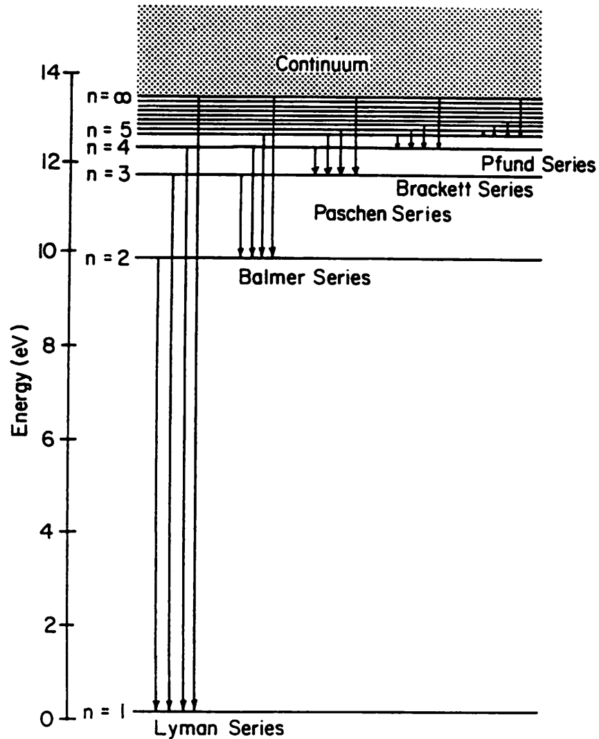
Fig. 1-4. Energy level diagram for the hydrogen atom showing the transitions that give rise to the observed spectral lines. (See Fig. 1-3.)
