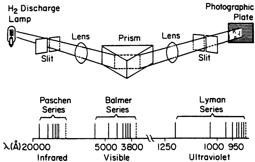
Fig. 1-2. A simple spectrograph.
